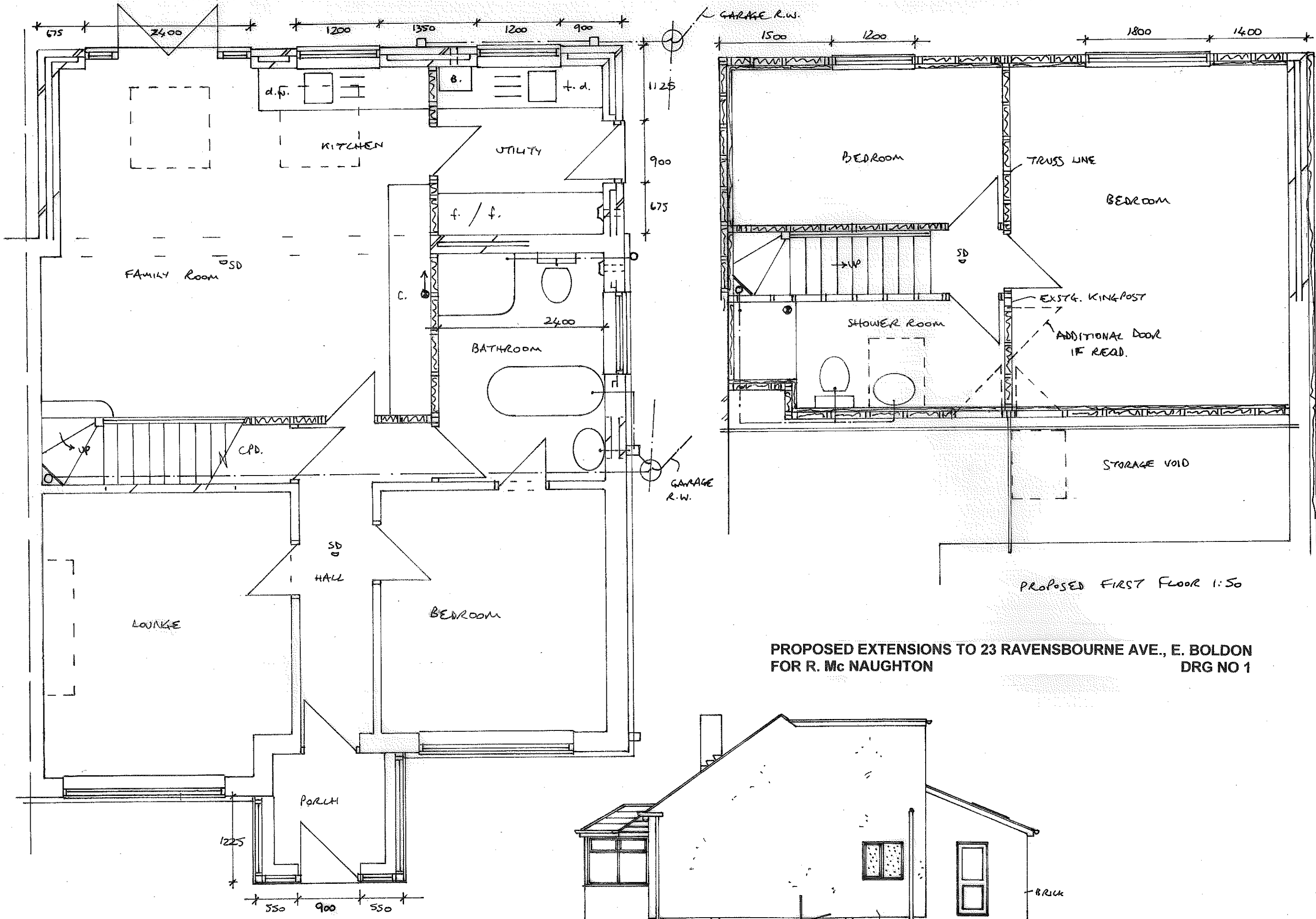
PROPOSED GROUND FLOOR 1:50
